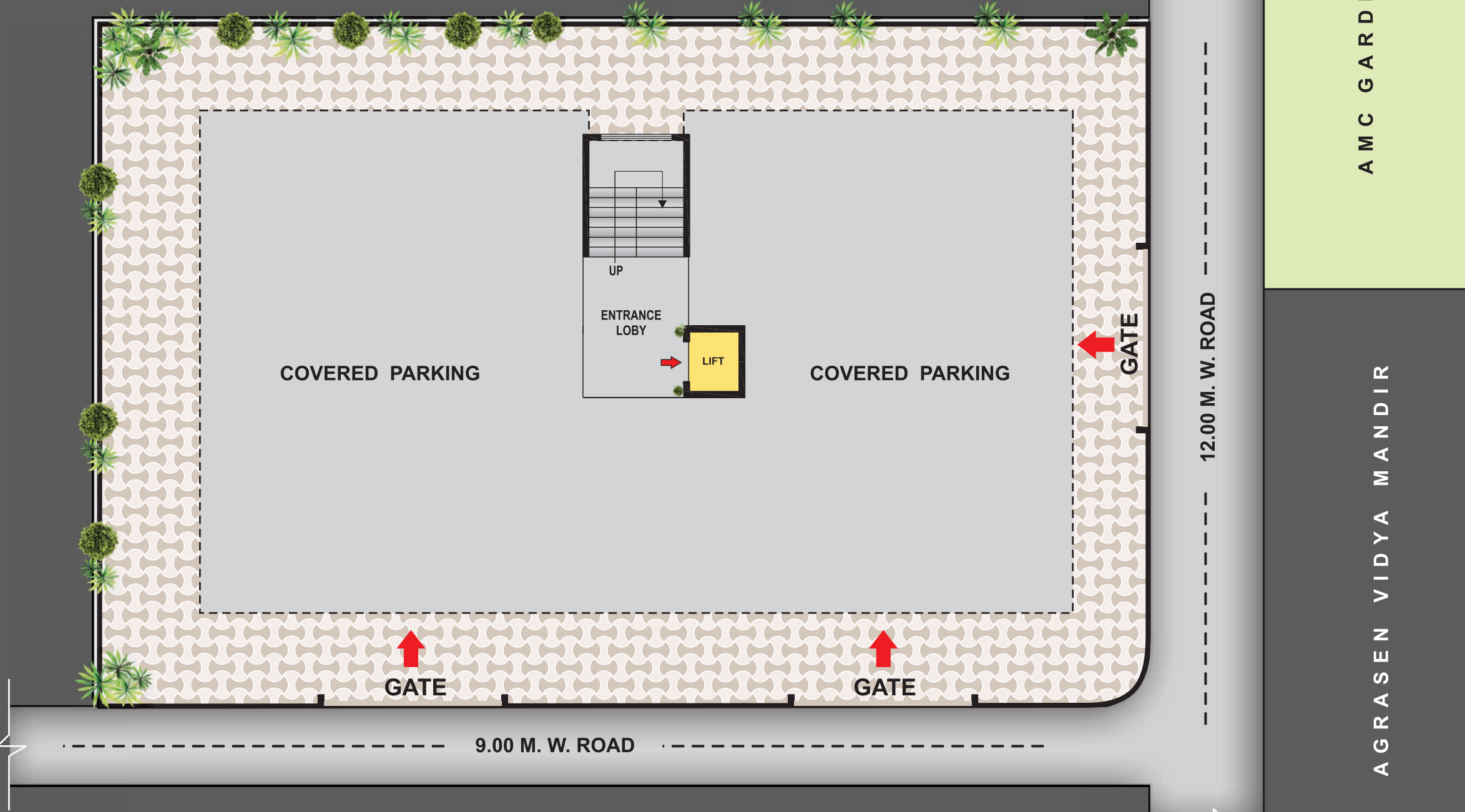
Parking Floor Plan
